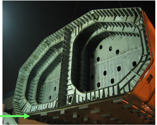
Gas carrier 23.000 m 3 with dehonit® / Perмали Tank Supports
