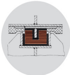
Fixed Bearing
