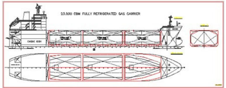
Gas carrier 23.000 m 3 with dehonit® / Perмали Tank Supports
